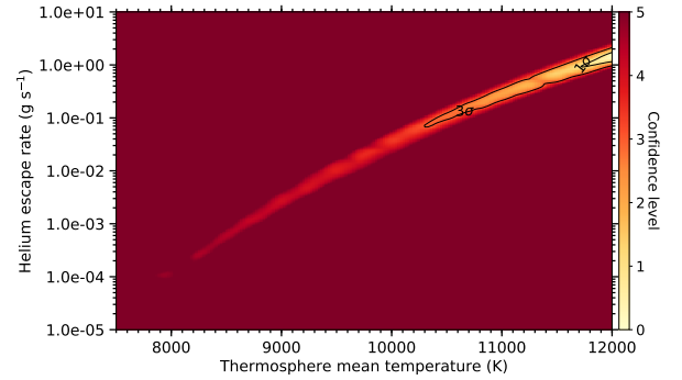
Fig. 13. Grid of \Delta\chi^2 (in confidence level) for the 1.2 R_p thermosphere extension. Black solid lines indicate the 1 and 3\sigma confidence contours.
