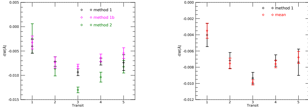
Fig. A.3. Comparison between the three fringing correction methods. The EW_{s,AB} values for the five nights ( x -axis) averaged between the contact point t_2 and t_3 are plotted. Left panel: results of the three methods (Method #1 in black, Method #1b in magenta, and Method #2 in green). Right panel: comparison between Method #1 and the weighted average of the three methods.
