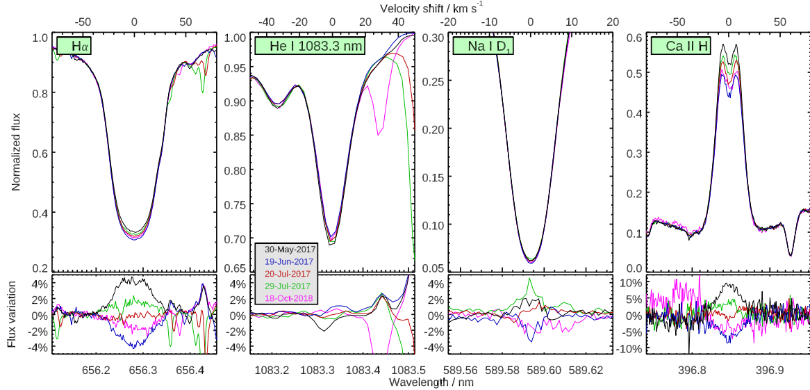
Fig. 7. Top panels: mean out-of-transit profiles of H\alpha , He I 1083.3 nm, Na I D_1 , and Ca II H (from left to right). The mean profile for each date is drawn with the same colour coding as in Fig. 1. Bottom panels: relative variation from the reference average profile (same colour coding).
