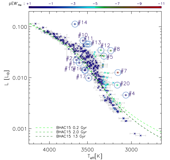
Fig. A.3. Same as Fig. 10, but using the pseudo equivalent width pEW'_{H\alpha} of Schöfer et al. (2019) for the color coding. Negative values of pEW'_{H\alpha} denote H\alpha emission. See Fig. 10 for the identification of the encircled stars.
