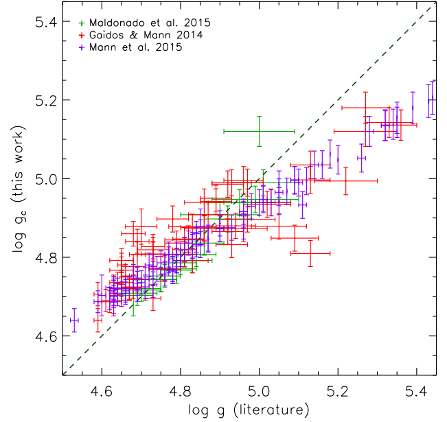
Fig. 7. Value of \log g_c calculated using M_{M-R} from Sect. 3.4 and using R from Sect. 3.3 against \log g from the literature.
