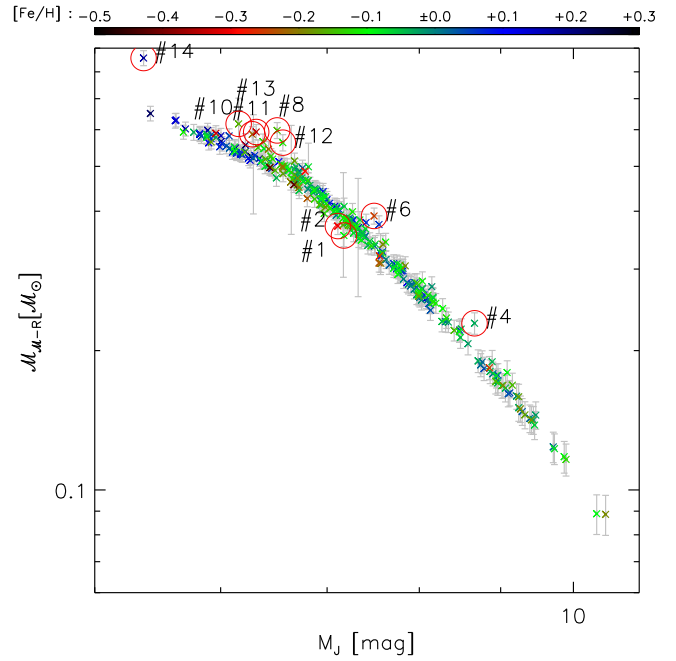
Fig. A.6. Value of M_{M-R} against absolute J magnitude M_J . Obvious outliers, and stars discussed in reference to this figure in Sect. 5.2, are encircled: #1=GJ 411 (J11033+359), #2=GJ 412A (J11054+435), #4=GJ 1235 (J19216+208), #6=GJ 15A (J00183+440), #8=1RXS J050156.7+010845 (J05019+011), #10=G 234-057 (J09133+688), #11=TYC 3529-1437-1 (J18174+483), #12=StKM 2-809 (J12156+526), #13=GJ 9520 (J15218+209), and #14=K2-33 (J16102-193). Outliers #11 and #13 lie almost on top of each other.
