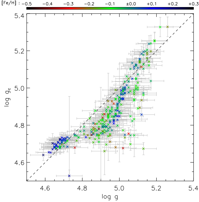
Fig. 6. Value of \log g_c calculated using M_{M-R} from Sect. 3.4 and using R from Sect. 3.3 against the spectroscopic \log g from Sect. 3.2.
