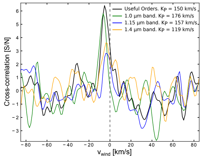
Fig. 8. CCFs with the largest significance obtained for the 1.0 \mu\text{m} band (green), 1.15 \mu\text{m} band (blue), and including all useful NIR orders (black). Also, the CCF for the 1.4 \mu\text{m} band with the largest significance peak in the positive K_p space is shown (orange). The vertical dashed line marks the zero velocity value.
