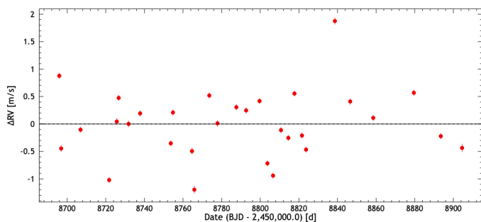
Fig. 23. Radial velocities obtained with ESPRESSO on \tau Cet. Only data obtained after the fiber upgrade are shown. Each data point corresponds to a nightly bin. In this case, the dispersion is of 0.58 \text{ m s}^{-1} .
