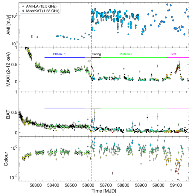
Figure 3. A zoom of Fig. 2, focusing on the most recent evolution of GRS 1915+105. The vertical dashed line marks the time of the change in the radio behaviour occurred on \approx MJD 58617.
