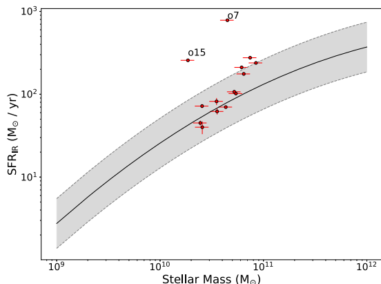
Figure 4. The \text{SFR}_{\text{IR}} from our sample of luminous IR galaxies plotted against the M_* , with the main sequence of Whitaker et al. (2014) represented by the grey shaded region. The solid line is the main sequence at z = 2.25 and the grey region represents 0.3 dex above and below this relation. Galaxies o7 and o15 fall within the starburst regime.
