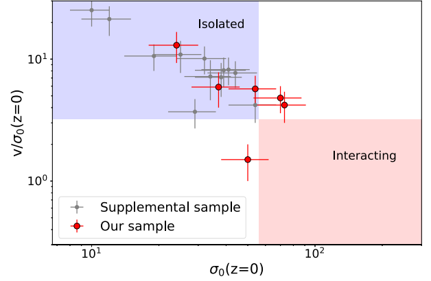
Figure 8. The dynamical ratio for the two sets of luminous IR galaxies: our sample (red) and the supplementary sample (grey). The dynamical ratio has been corrected for the redshift evolution in velocity dispersion as discussed in Section 4.4 The blue/red boxes represent typical values seen in isolated discs/interactions with threshold values of \sigma_0 < 56 \text{ km s}^{-1} and v_{\text{rot}}/\sigma_0 > 3.2 for isolated discs. 3/6 of our sample appear to be isolated with all 12 of the supplementary sample falling within the boundaries of an isolated galaxy. Galaxies falling within the white areas cannot be determined using this method and can only be categorized by relaxing one of the assumptions.
