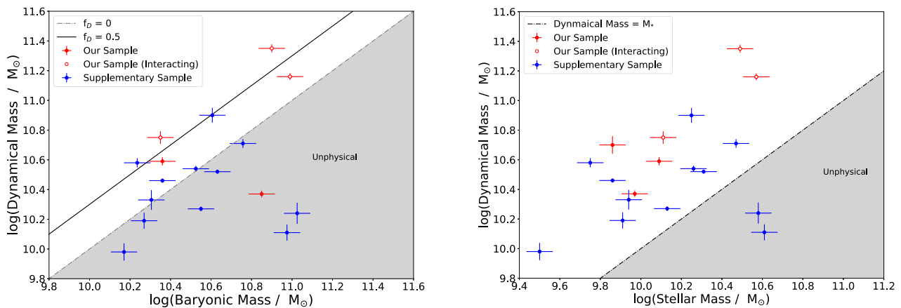
Figure 9. Plot of the dynamical mass versus baryonic mass within one R_E (left) with the grey area representing unphysical values where the baryonic mass exceeds the dynamical mass. Dark matter fraction increases with vertical height above the dashed line, where dynamical mass equals baryonic mass, and the black solid line indicates where the dark matter fraction equals 50 per cent. Three of our sample fall into the dark-matter-dominated region (dark matter fraction > 50 per cent), with eight of our sample in the unphysical region. The unphysical values are mainly caused by our estimate of gas fraction, as discussed in Section 4.5, which can be seen when we remove the gas mass and plot stellar mass versus dynamical mass within one R_E (right). Further reasons for unphysical values are discussed in Section 4.5. The three galaxies (o3, o14, and o16) that passed only one of our two kinematic criteria for an isolated disc in Section 4.4 are included as the interacting subsample and these may be an overestimate of the dynamical mass. The left plot only contains five data points for our KMOS sample as we were unable to estimate a baryonic mass for galaxy o8.
