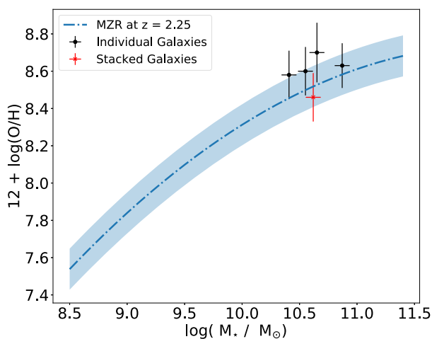
Figure 12. The position of our four galaxies with [\text{N II}] 6583 \text{ \AA} detection, and the composite spectrum, with respect to the MZR. The track represents the values expected for z = 2.25 taken from Tacconi et al. (2018), and the scatter in this relation is \sim 0.1 dex. This plot indicates our four detections are not metal deficient, with the composite spectrum also lying within the scatter of the MZR.
