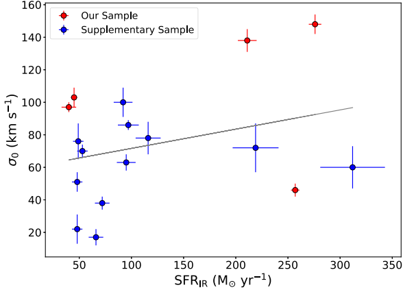
Figure 10. Intrinsic velocity dispersion plotted against SFR (left) and baryonic masses (right) of our galaxies. There is a weak correlation for both \sigma_0 versus SFR and \sigma_0 versus baryonic mass with a Pearson's \rho = 0.37 (P-value = 0.23) and \rho = 0.37 (P-value = 0.13) for the SFR and baryonic mass, respectively, although neither is statistically significant. Galaxy o8 could not be fitted with an IR SED so we do not have an \text{SFR}_{\text{IR}} for this galaxy, giving only five data points in our sample for the left plot.
