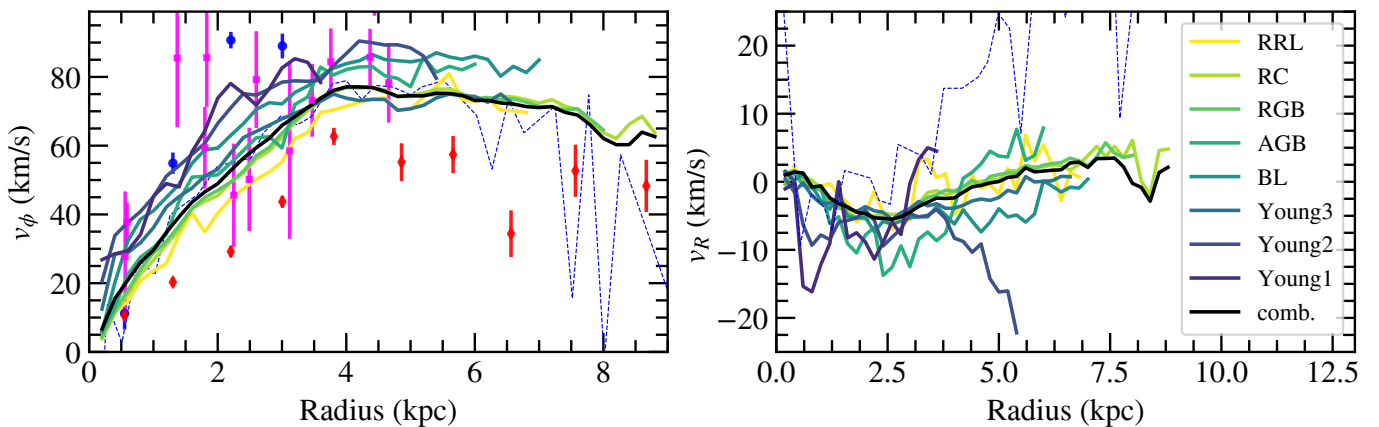
Fig. 14. Stellar velocity curves of the LMC. Left and right panels: rotation curves and radial motions, respectively. Coloured lines are for the eight evolutionary phases and the combined sample, as given by the legend. In the left panel, blue circles, red diamonds and magenta squares are the rotation velocities for the samples of younger and older stars from line-of-sight spectroscopic and HST astrometric measurements published in van der Marel & Kallivayalil (2014) . The dashed blue lines are the tangential and radial velocity profiles derived by Wan et al. (2020) from Gaia DR2 astrometry.
