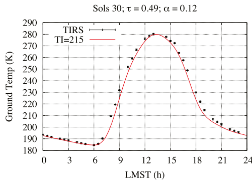
Figure 5. Ground temperature as a function of Local Mean Solar Times on sol 30 ( L_s \sim 20^\circ ) measured by Thermal Infrared Sensor (black) and solved numerically from Equations 3–5 with a best-fitting value of TI = 215 SI units. The cool bias in the numerical values during early and late daytime hours is caused by the assumption of homogeneous terrain, which we take in this study for the sake of simplicity. Note that the best-fitting value of TI obtained by Single Column Model (SCM) is 225 SI units (Figure 4). A similar good match in TI between SCM and MEDA observations (Equations 3–5) was obtained for other sols.
