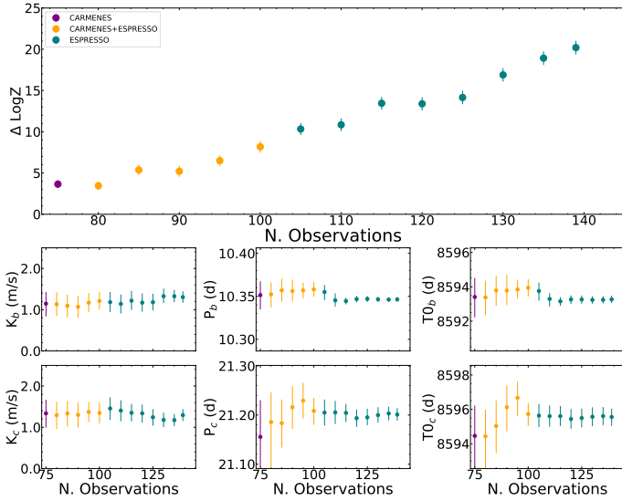
Fig. 14. Signal stability test. Top panel: evolution of the difference in Bayesian evidence ( \Delta \text{Log Z} ) of the 2-planet model against an activity-only model. Bottom panels: evolution of the parameters of the two sinusoids. The colours of the points show which data are added at each step.
